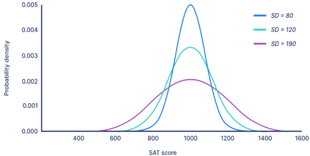
Normal distributions with different standard deviations
